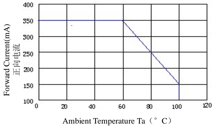
4. Forward Current Derating Curve, Derating based on T_{max}=125^{\circ}C 正向电流降额曲线, 以 T_{max}=125^{\circ}C 为基准
