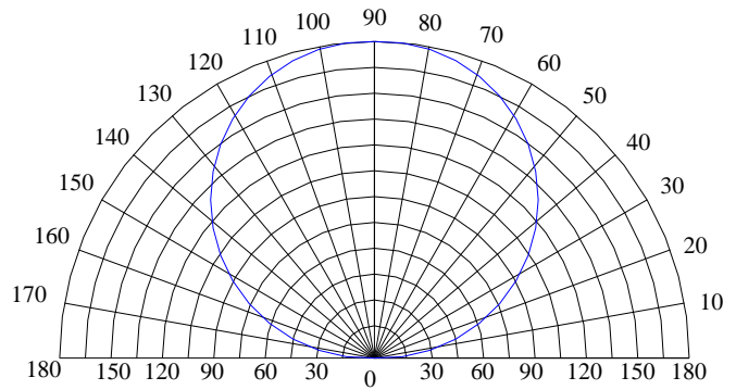
2. Typical Light-Emitting Angle Radiation Pattern 典型发光角度辐射图
