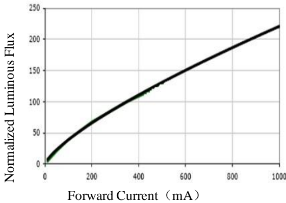
3. Forward Current vs. Relative Luminous Flux Curve 正向电流与相对光通量曲线图
