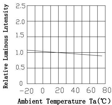
Ambient Temperature VS. Relative Intensity
